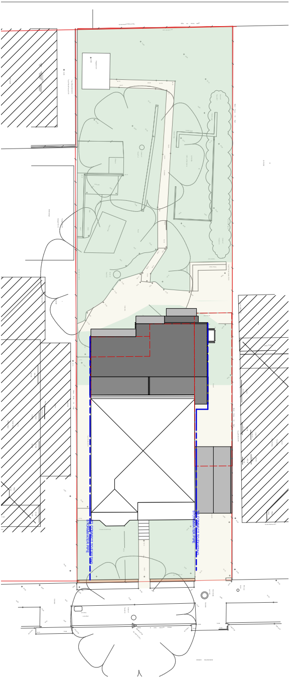
1 STORMWATER CONCEPT PLAN Scale: 1:200
